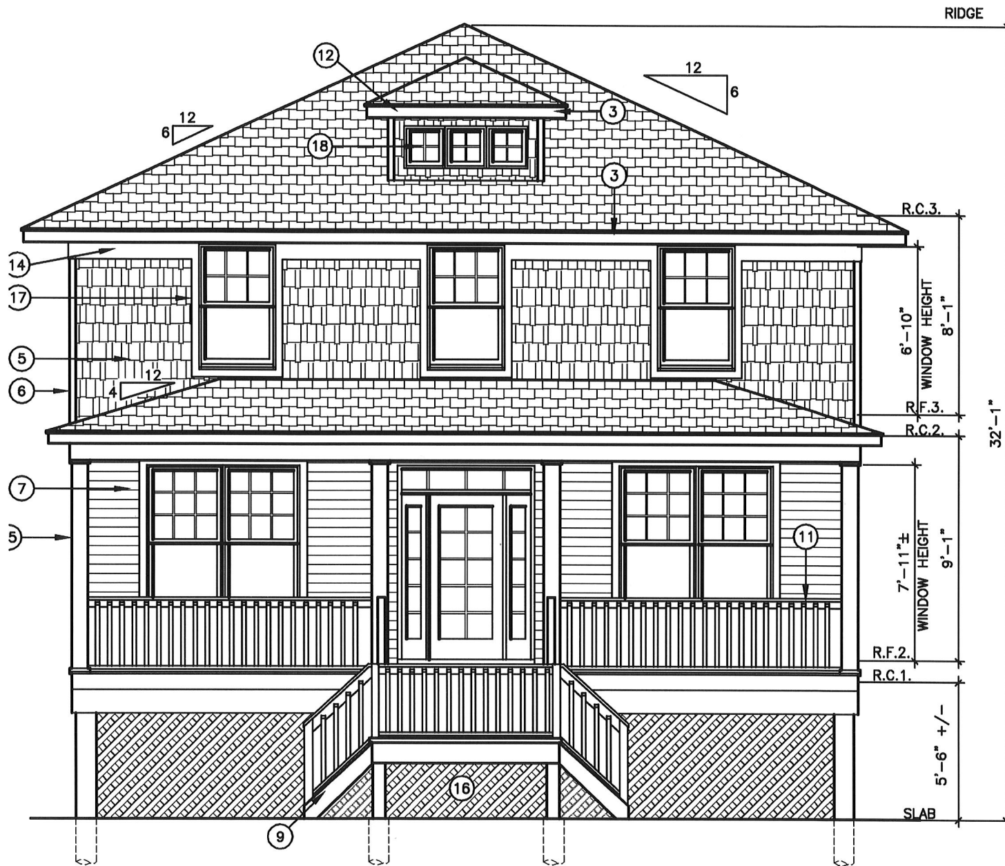
FRONT ELEVATION
